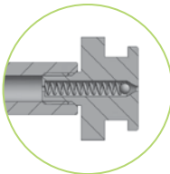
403- ND-Flachkopfnippel LP pan head nipple
