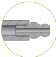
409- OD-Kegelnippel WP round head nipple
